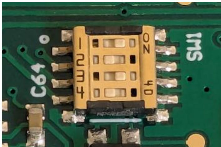
Figure 28: Version 2 of the ASM external Analog-Box with toggle switches: switch 1 & 3 need to be set to "ON" for DC operation on Channel 1 & Channel 2
